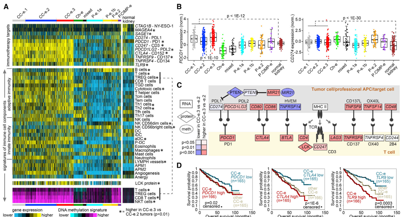
Figure 7. Immune-Checkpoint-Related Differences across RCC Genomic Subtypes
